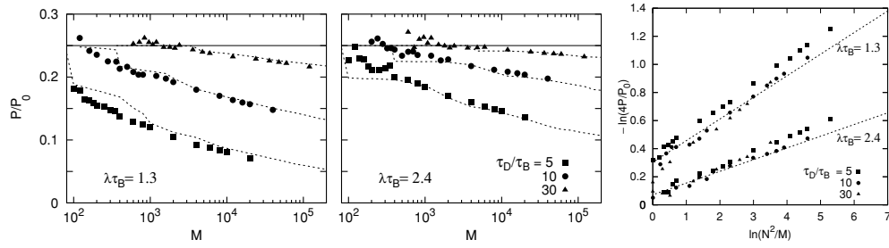
Figure 3. Left and middle panels: dependence of the shot noise on the semiclassical parameter M \sim \tau_H/\tau_B for two different Lyapunov exponents \lambda and three different dwell times \tau_D of the open kicked rotator (as indicated in the plots). The solid line is the prediction from RMT. The dashed lines are obtained from a semiclassical estimate of the number of deterministic transport channels [38]. Right panel: rescaled data in a double-logarithmic plot, together with lines of slope 1/\lambda\tau_D . The figures have been adapted from [31].
